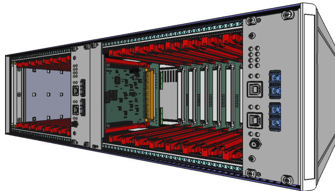
Figure 4: View of the SPK84-D Platform (dual-backplane option). Two SK810 Interfaces Controller modules are used here to communicate with up to 16 single-wide instruments. Since the SKP84-D is equipped with two distinct backplanes, it actually behaves like two SPK42 platforms assembled in a single case.
